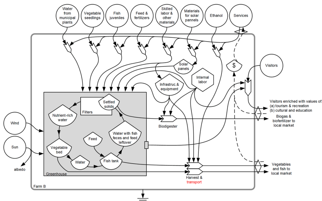
Fig. 2. Energy diagram of the aquaponics system in Farm B.
